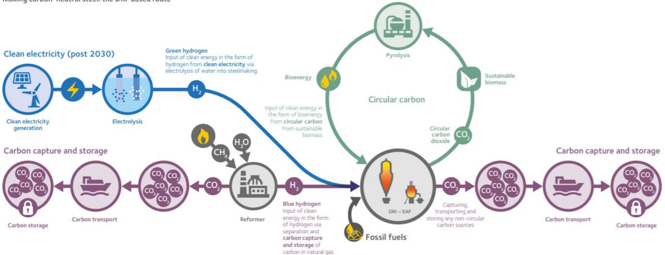
Making carbon-neutral steel: the DRI-based route
